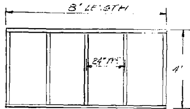
RETAINING WALL SUBASSEMBLY 1 SHEET OF 1/2" PLYWOOD 5-2"x4" STUDS 2-2"x4" STUD PLATES 6 REQUIRED
